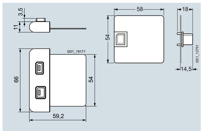
7LF4941-0 USB adapter
