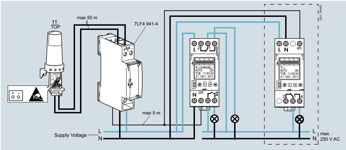
Expert GPS digital time switches (7LF4541, 7LF4542) with GPS antenna (7LF4941-5) and power supply unit for GPS antenna (7LF4941-4)
