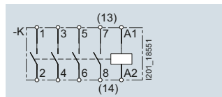
5TT5030 5TT5040 5TT5050
